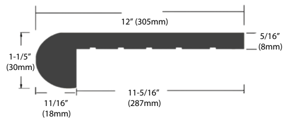
STAIR TREAD
